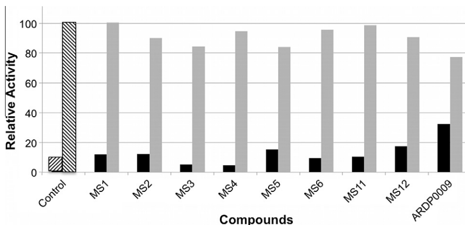
Fig. 1. Relative activity of DEN2V NS2B-NS3pro. The black bars display the averaged relative fluorescence of the protease reaction in the presence of inhibitors. The fluorescence intensity was normalized to the averaged signal produced by the protease reaction without inhibitor (hatched bar, second from the left). The gray bars display the averaged relative fluorescence of AMC in the presence of inhibitors, normalized to the signal produced by AMC alone. The first hatched bar on the left-hand side is a control containing substrate alone.
