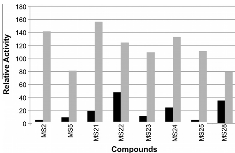
Fig. 2. Relative activity of DEN2V NS2B-NS3pro. The black bars display the averaged relative fluorescence of the protease reaction in the presence of inhibitors. The fluorescence intensity was normalized to the averaged signal produced by the protease reaction without inhibitor. The gray bars display the averaged relative fluorescence of trypsin in the presence of inhibitors, normalized to the signal produced by trypsin alone.
