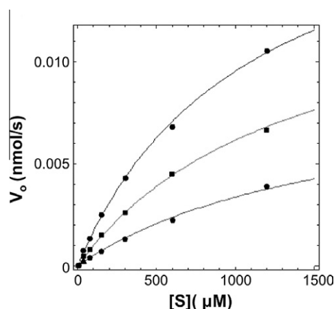
Fig. 4. Representative curve for inhibitor MS28 (alexidine hydrochloride), which was modeled as having a mixed inhibition mechanism against DEN2V NS2B-NS3pro. Concentrations of MS28 tested were 0 (circles, top curve), 30 (squares, middle curve), and 100 (pentagons, lower curve) \mu\text{M} . Data were analyzed with the program Dynafit, with curves calculated from global fitting to the data points. Error bars were within the dimensions of the data points.
