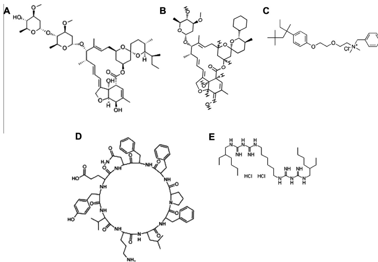
Fig. 5. Chemical structures for lead DEN2V protease inhibitors: (A) ivermectin (MS21), (B) selamectin (MS24), (C) methylbenzethonium chloride (MS22), (D) tyrothricin (MS23), and (E) alexidine hydrochloride (MS28).
