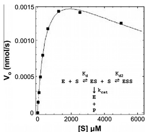
Fig. 3. DEN2V protease reaction with the small peptide substrate Boc-Gly-Arg-Arg-AMC demonstrated Michaelis-Menten kinetics with substrate inhibition. The model curve was produced with the program Dynafit, which optimized the kinetic parameters in a substrate inhibition model (insert) to best fit the data points.
