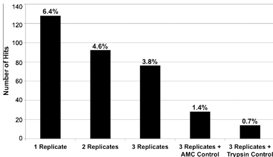
Fig. 6. Hit rate as a function of replicate number and inclusion of AMC and trypsin internal controls.
